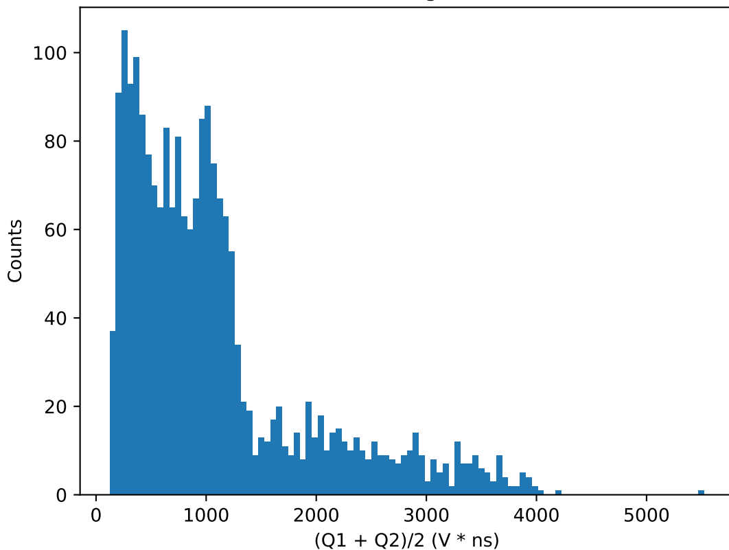
(Q1 + Q2)/2 histogram for 43.0V
