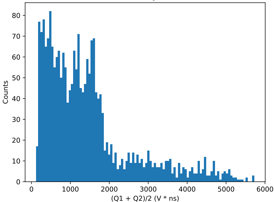
(Q1 + Q2)/2 histogram for 44.0V
