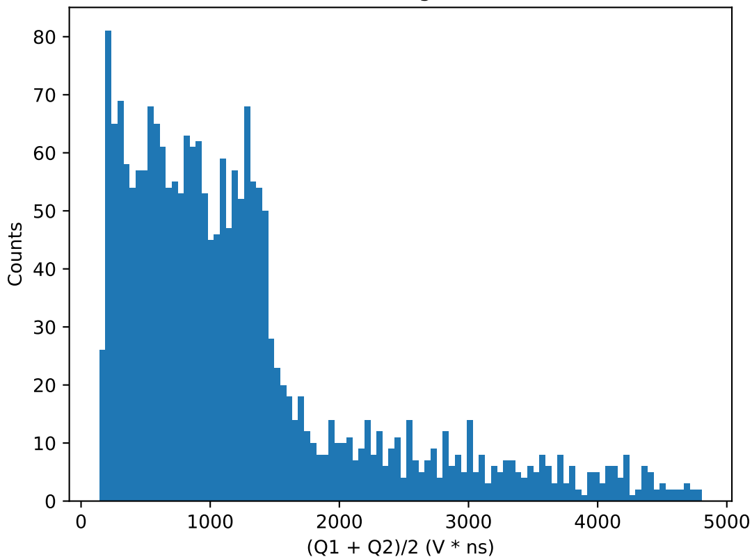
(Q1 + Q2)/2 histogram for 43.5V
