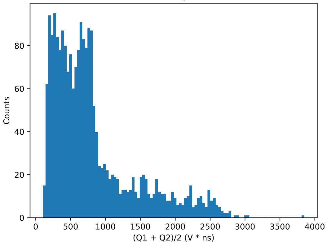
(Q1 + Q2)/2 histogram for 42.0V
