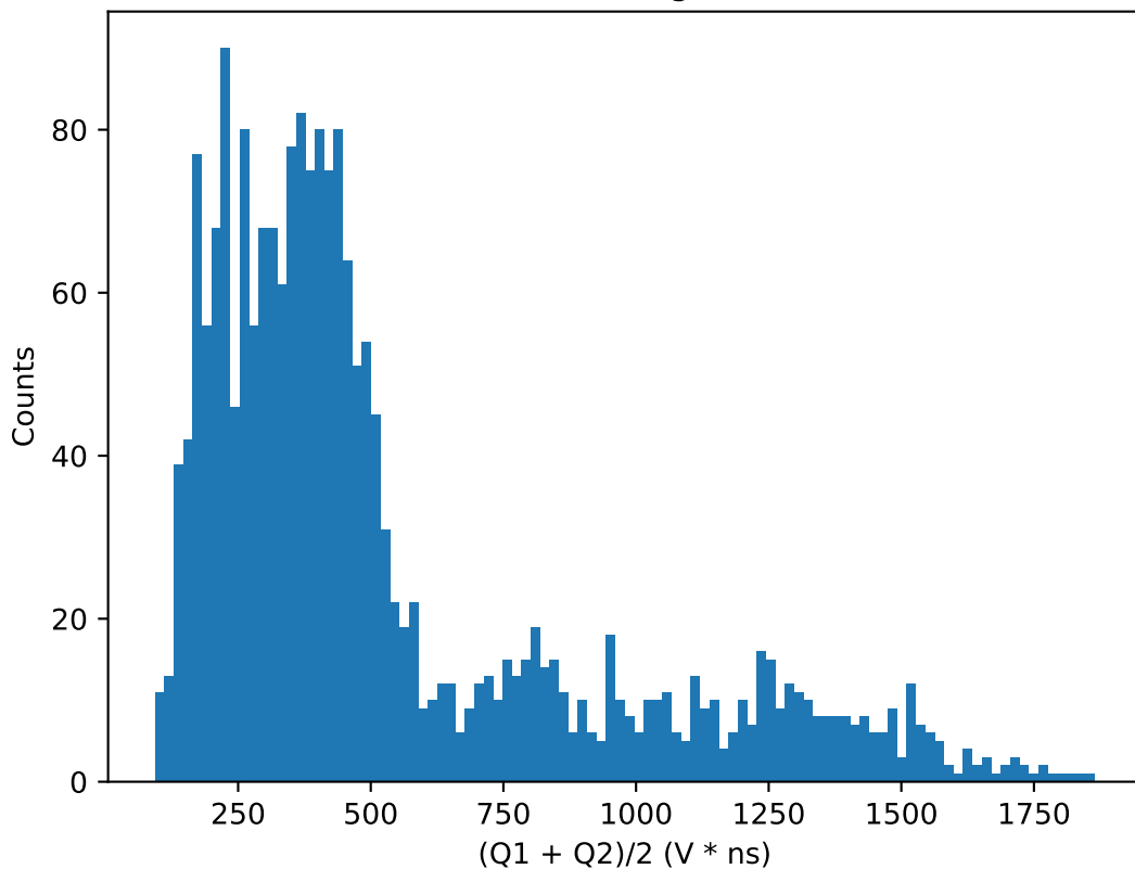
(Q1 + Q2)/2 histogram for 41V
