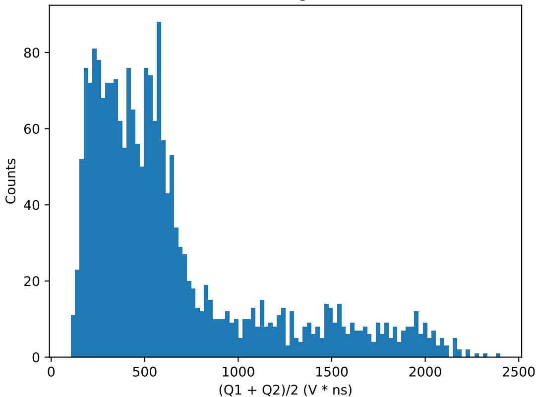
(Q1 + Q2)/2 histogram for 41.5V
