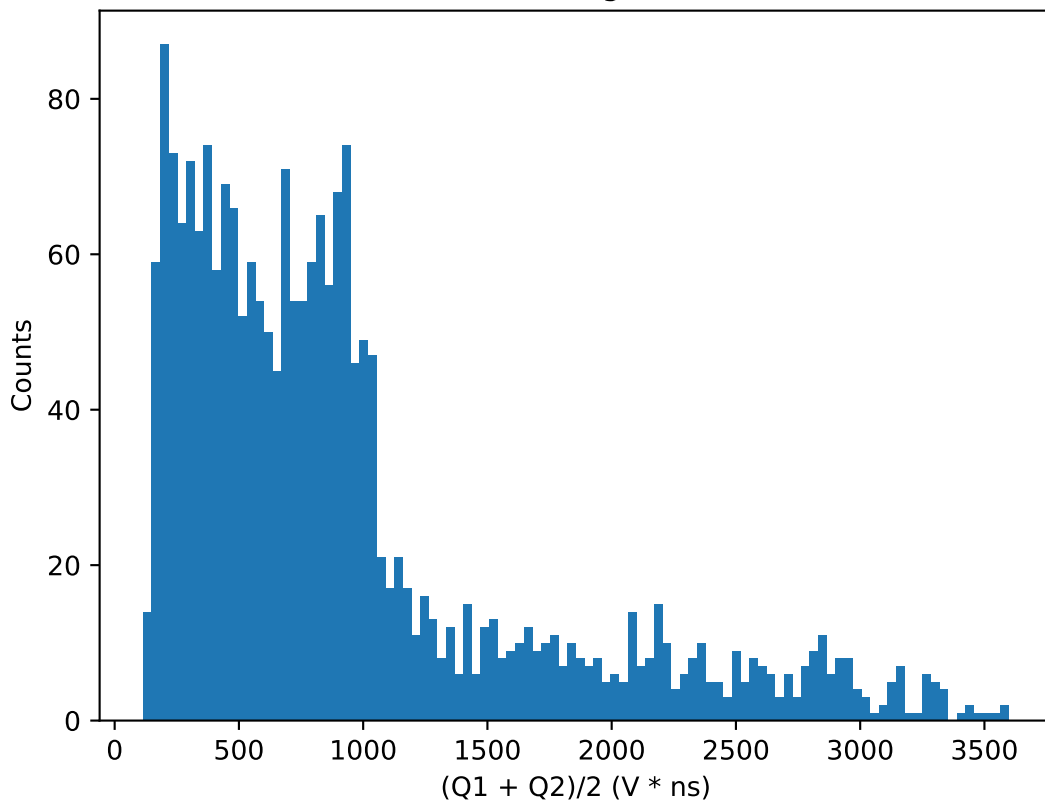
(Q1 + Q2)/2 histogram for 42.5V
