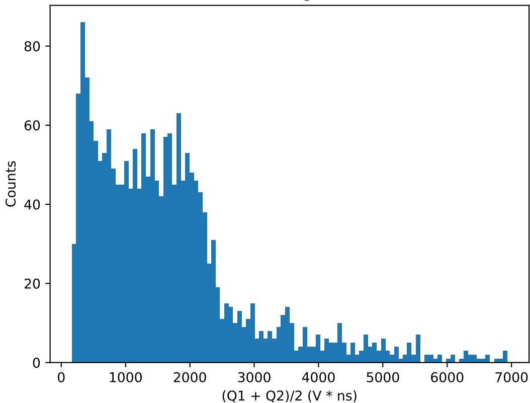
(Q1 + Q2)/2 histogram for 45.0V
